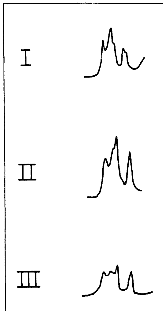
Fig. 2.—Variation in the H_1' - H_5' region of uridine.
