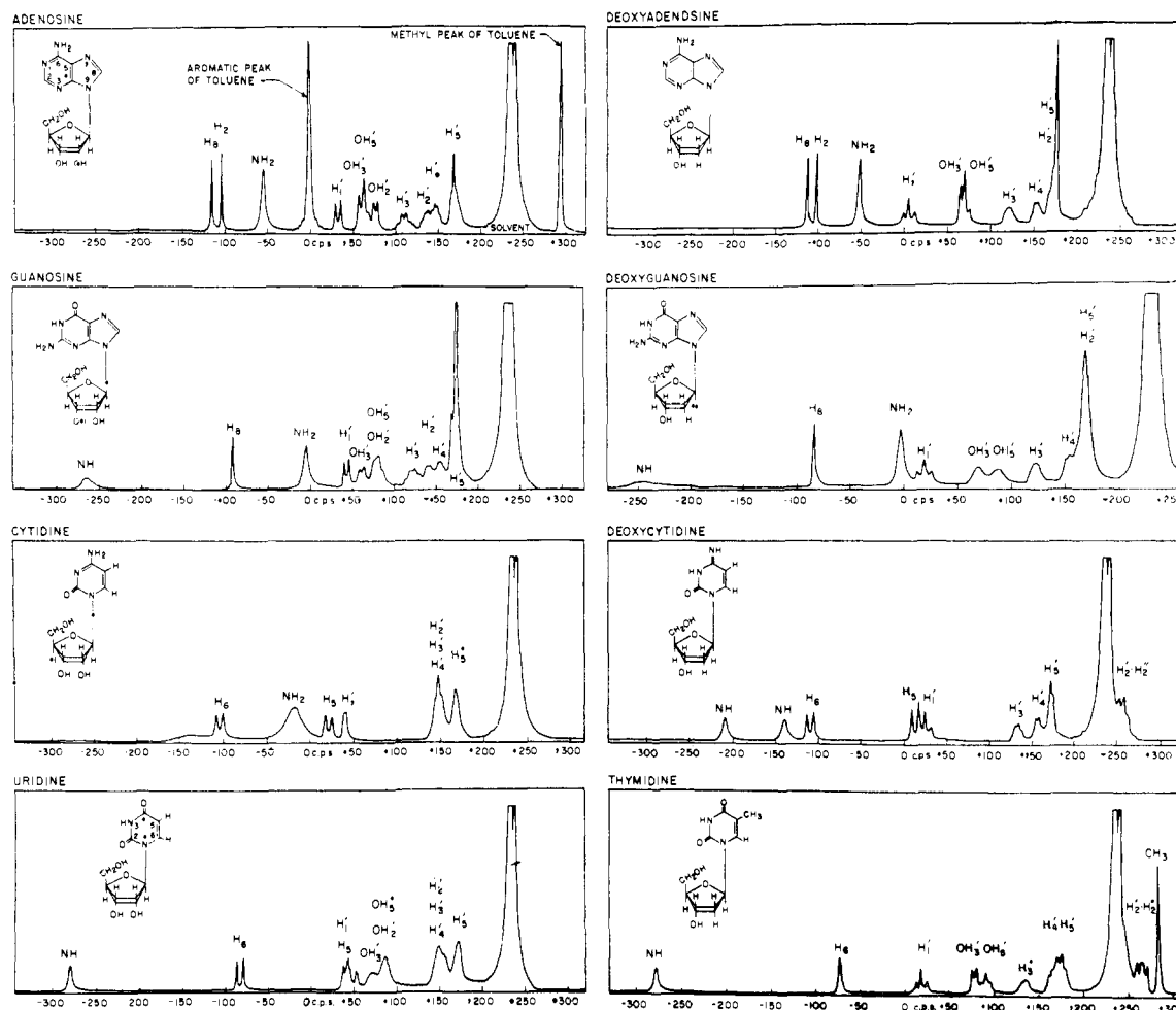
Fig. 1.—60 Mc. n.m.r. spectra of ribose and deoxyribose nucleosides in dimethyl sulfoxide; field increases from left to right; sweep rate 174 c.p.s. min. -1 , H_1 field 60 db. attenuation below 0.5 watt, frequency response 100 c.p.s. Toluene reference peaks included in the adenosine spectrum. Primed numbers refer always to ribose ring.
