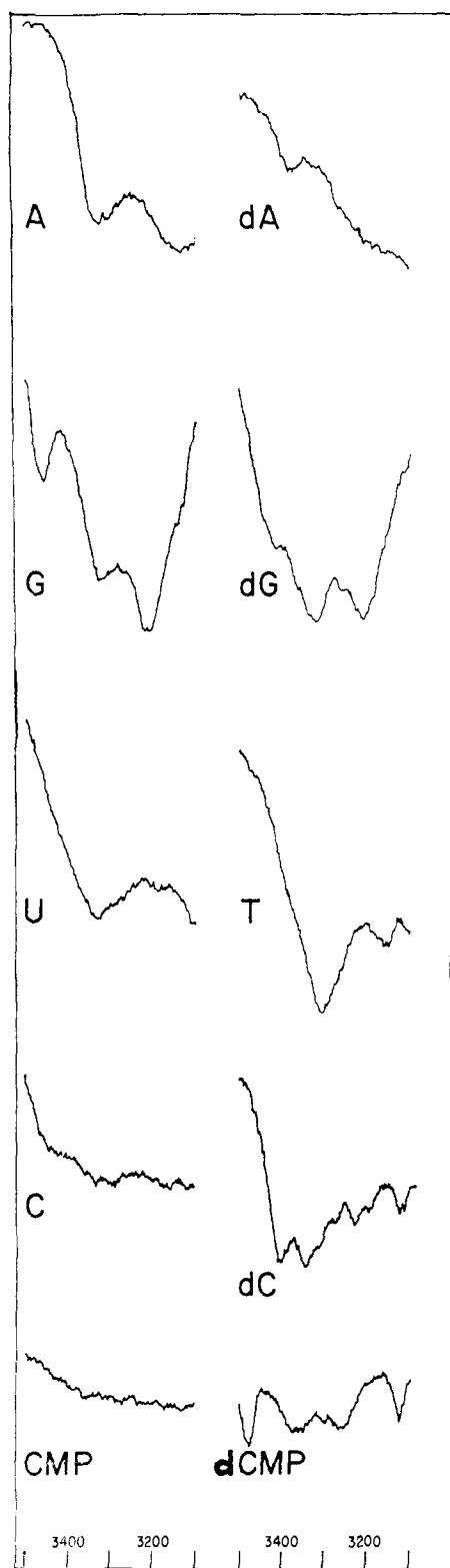
Fig. 5.—Infrared spectra of the NH stretching frequency region in \text{cm}^{-1} of Nujol emulsions of: A, adenosine; dA, deoxyadenosine; G, guanosine; dG, deoxyguanosine; C, cytidine; dC, deoxycytidine; U, uridine; T, thymidine; CMP-5'; and dCMP-5'.
