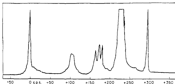
Fig. 3.—Ribose in dimethyl sulfoxide. Toluene reference peaks are included. Conditions are the same as in Fig. 1.
