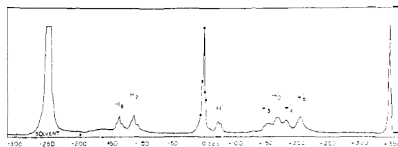
Fig. 4.—Adenosine in trifluoroacetic acid; conditions same as in Fig. 1.
